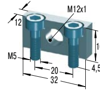
MB12SC2 Montageblock
